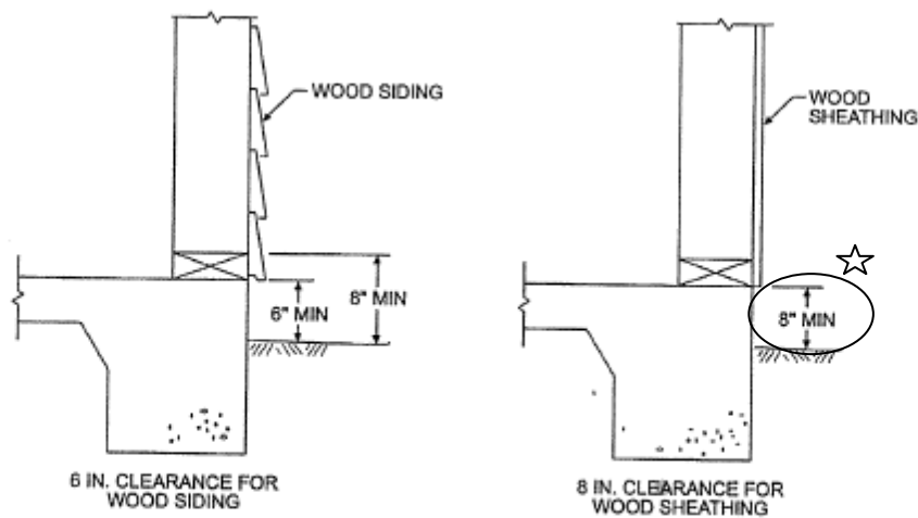
CLEARANCE FOR WOOD SIDING AND SHEATHING FIGURE 23-13
