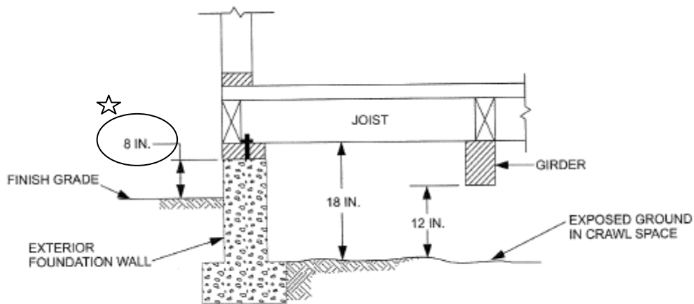
Figure 2304.11.2.1 WOOD-FRAMING CLEARANCES
